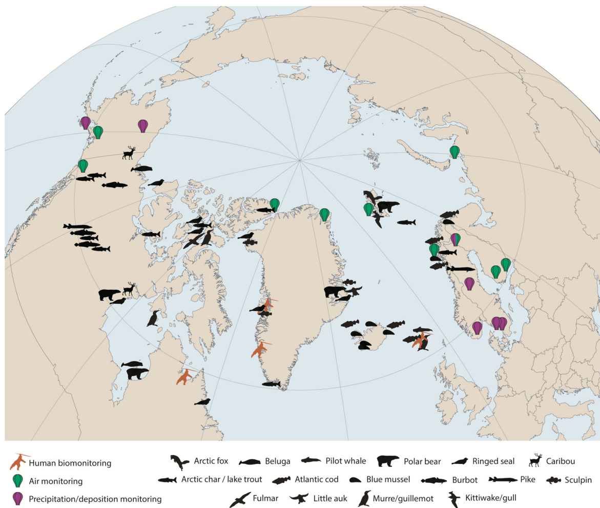
Fig. 1. Map of sampling locations for available time series of total mercury (THg) in biota included in the 2021 AMAP Mercury Assessment and the present study (see SI Table A1 for details on biota). Human biomonitoring, air and precipitation/deposition sites are described in other articles in this special issue. Figure reproduced with permission from AMAP (2021), with modification.
