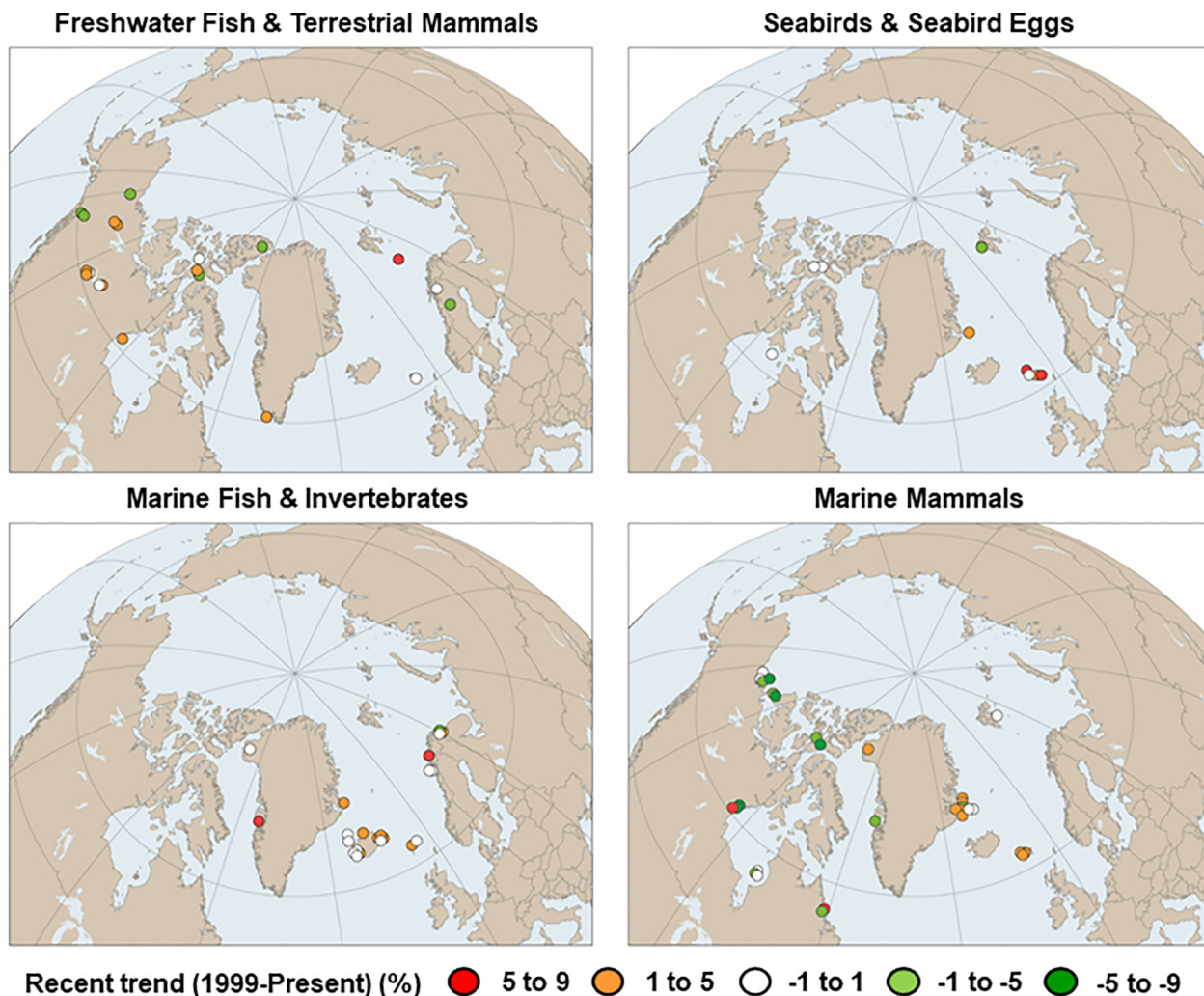
Fig. 3. Geographical patterns in recent (last 20 years) trends of THg concentrations in tissues of biota, where trends were significant and/or time series were of a statistical power \geq 80\% . The figures show freshwater fish and terrestrial mammals (top left); seabirds (top right); marine invertebrates (mussels) and marine fish (bottom left) and marine mammals (bottom right). Overlapping symbols have been dispersed to make them visible, resulting in clusters of points around some monitoring locations where trends are available for multiple time series (see SI Table A2). Figure reproduced with permission from AMAP (2021), with modification.
