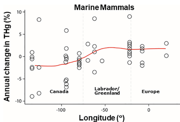
Fig. 6. Annual change of total mercury (THg, %) over time in marine mammals as a function of longitude ( ^\circ ). Data points represent the recent trends (1999–present) for an individual time series. The red line represents the non-linear relationship that best describes the pattern of trends in marine mammals (trend values are available in SI Table A2). Figure reproduced with permission from AMAP (2021).
