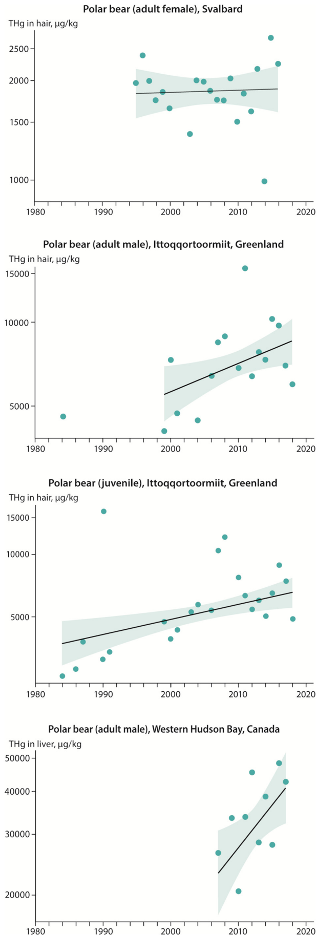
Fig. 5. Selected temporal trends and 95% confidence bands of THg concentrations in hair and liver ( \mu\text{g}/\text{kg} ) of polar bears. Bears are from Svalbard (hair of adult females, dry weight), Ittoqqortoormiit, Greenland (hair of adult males and juveniles, dry weight), and Western Hudson Bay, Canada (liver of adult males, wet weight) (see SI Table A2). Data points are annual medians of \log_e concentrations, with the y-axis back-transformed for visualization. Figure reproduced with permission from AMAP (2021).
