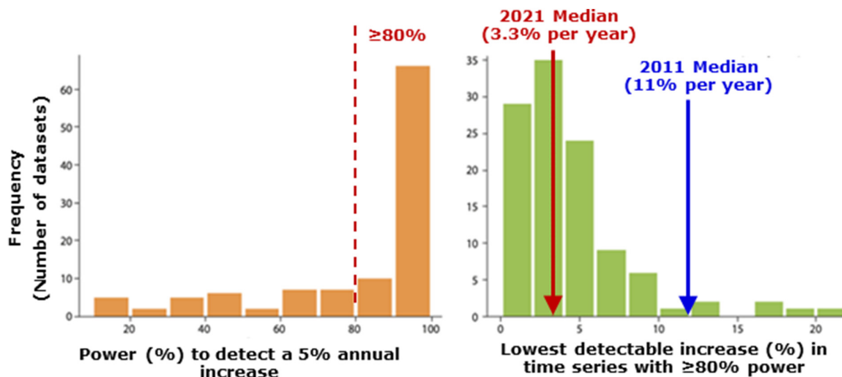
Fig. 2. Histogram of the power to detect a 5% annual increase ( \geq 80\% power indicated by dashed line, left panel) and the lowest annual increase detectable with \geq 80\% power (right panel) given the current configuration of years in the available THg time series. Figure reproduced with permission from AMAP (2021), with modification.
